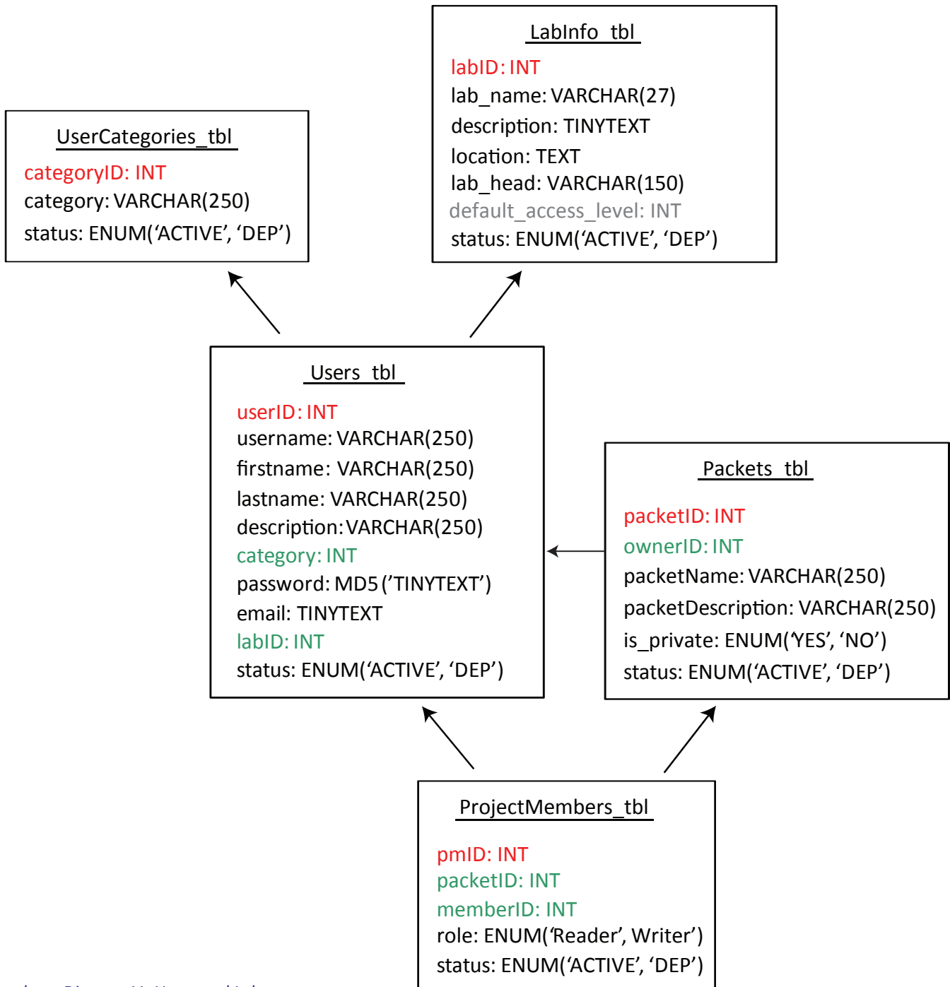
Database Diagram V. Users and Labs
